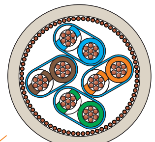
S/FTP
